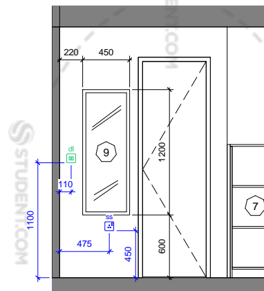
Elevation C - LH Room 1 : 50
