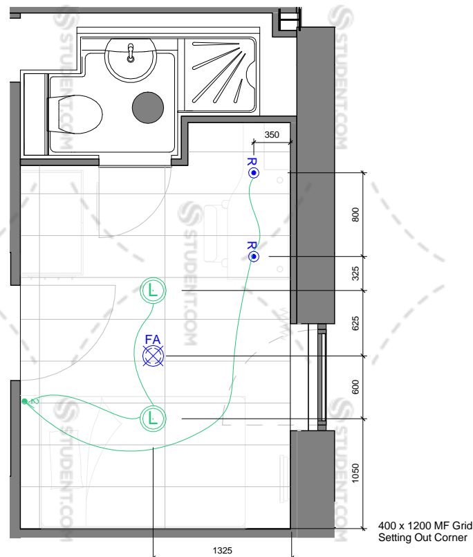
SB_11 - Reflected Ceiling Plan
