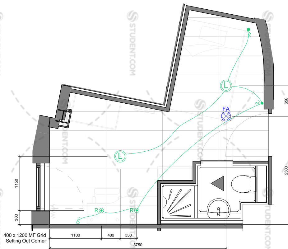
SB_6 - Reflected Ceiling Plan
