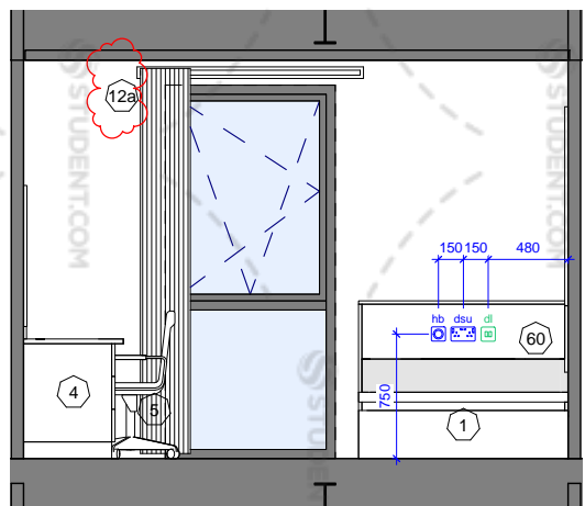
SB_2 - Elevation B 1 : 50
