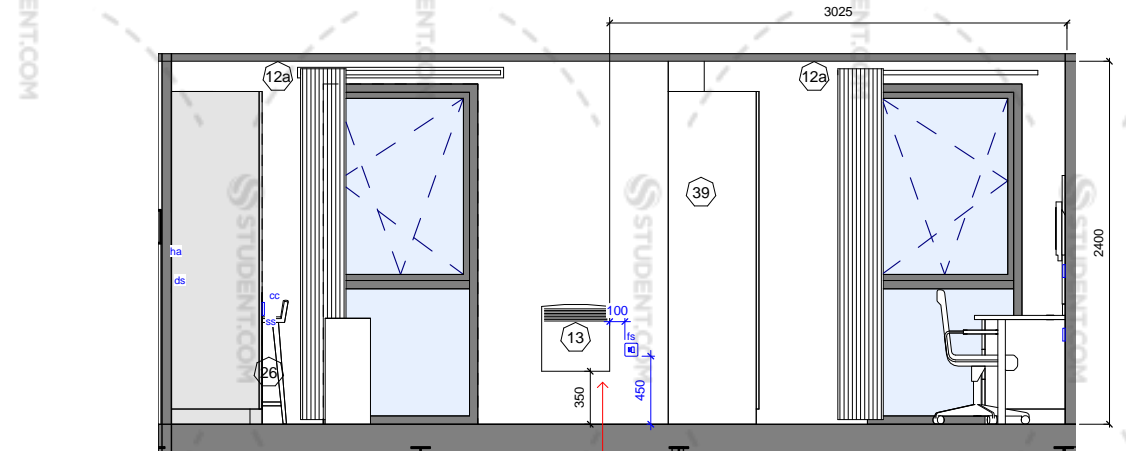
SB_13 - Elevation A
