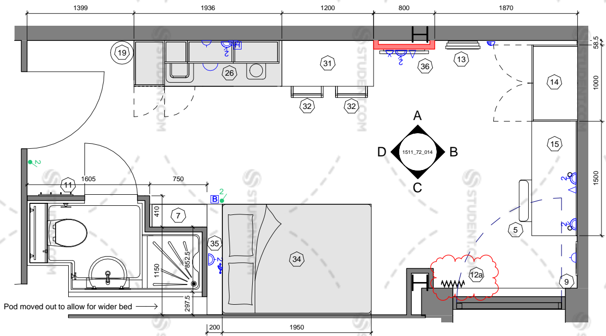
SB_14 - Plan View 1 : 50
