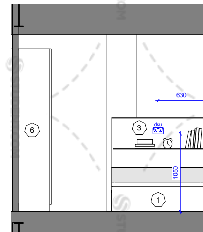
SB_1 - Elevation B
