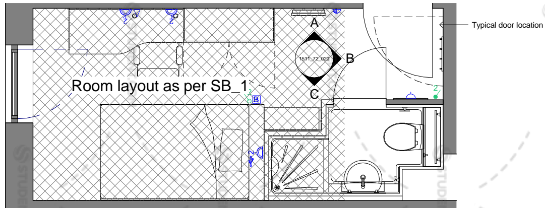
SB_1 - Plan View (Door Variant)
