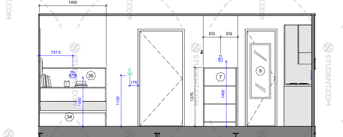
SB_13 - Elevation C
