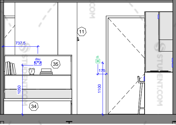
SB_14 - Elevation D 1 : 50
