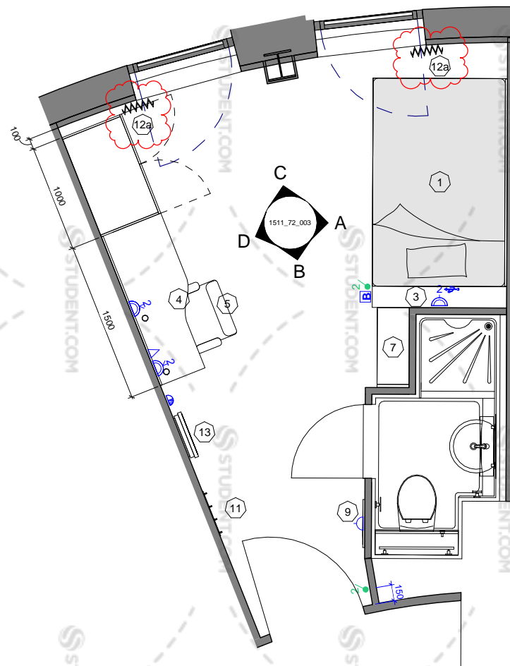
SB_3 - Plan View
