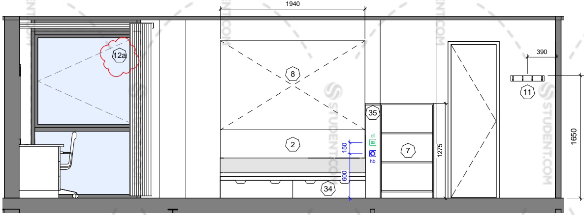
SB_14 - Elevation C 1 : 50
