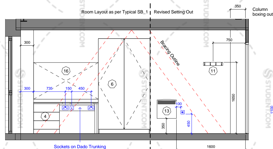
Elevation A - Left Hand Room 1 : 50
