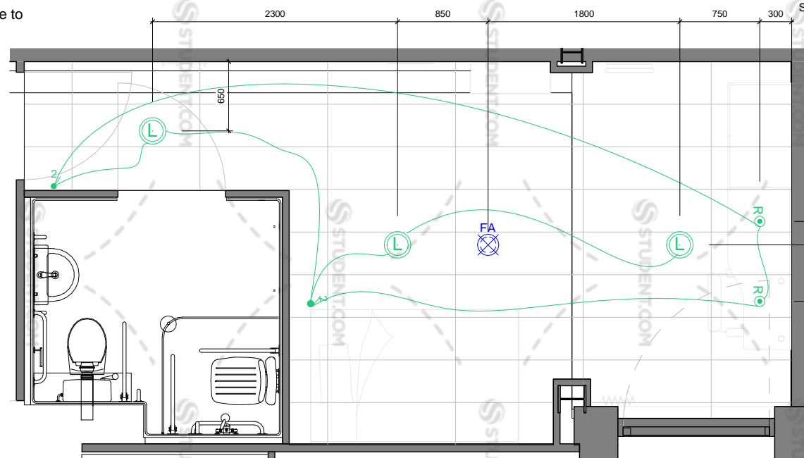
SB_12 - Reflected Ceiling Plan
