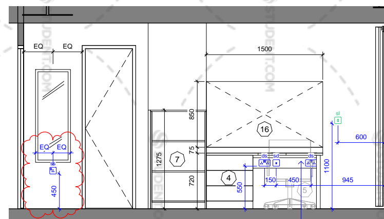
SB_6 - Elevation C
