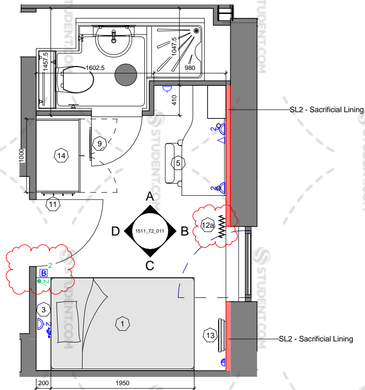
SB_11 - Plan View
