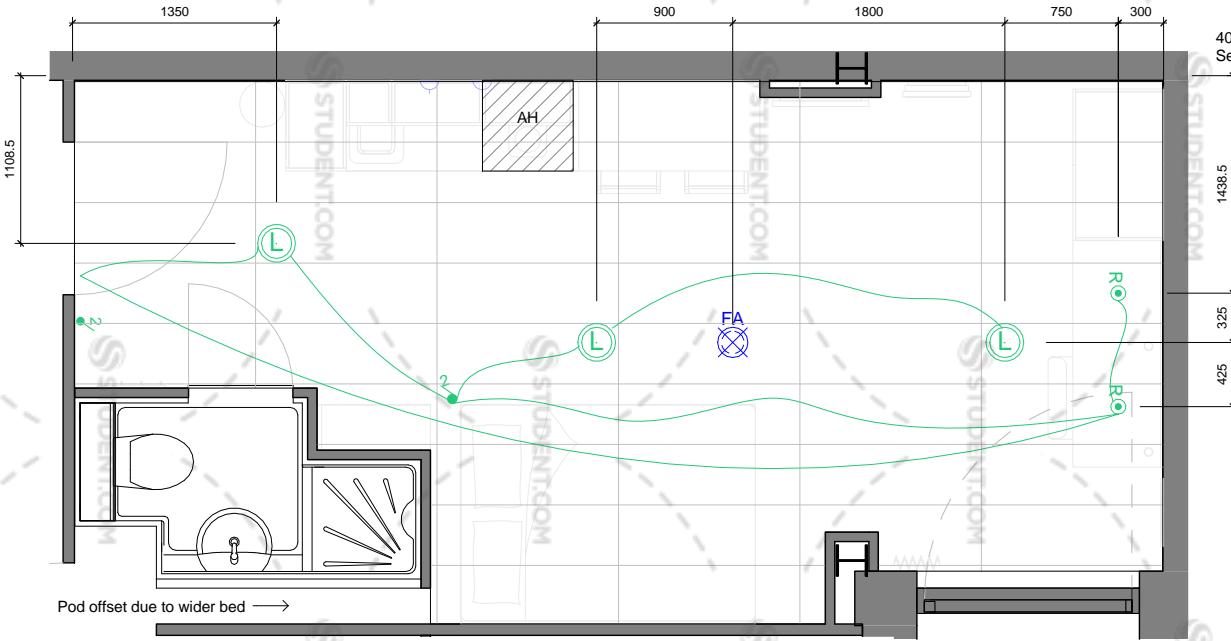
SB_14 - Reflected Ceiling Plan 1 : 50
