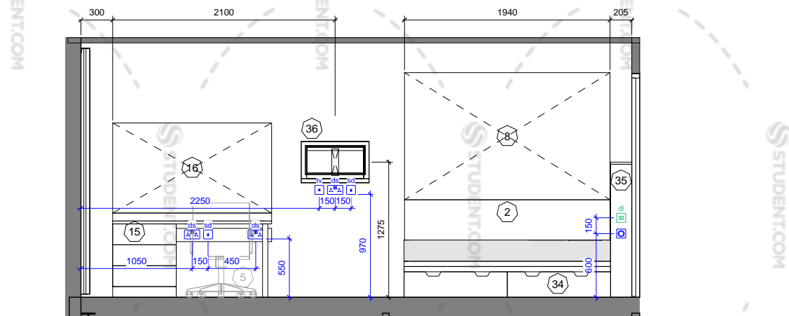
SB_13 - Elevation B
