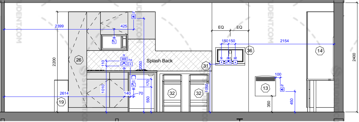
SB_14 - Elevation A 1 : 50
