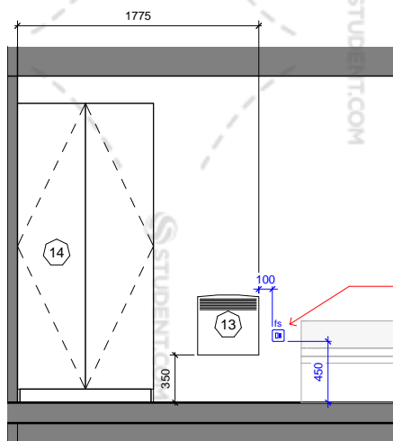
SB_2 - Elevation C (Mirror) 1 : 50
