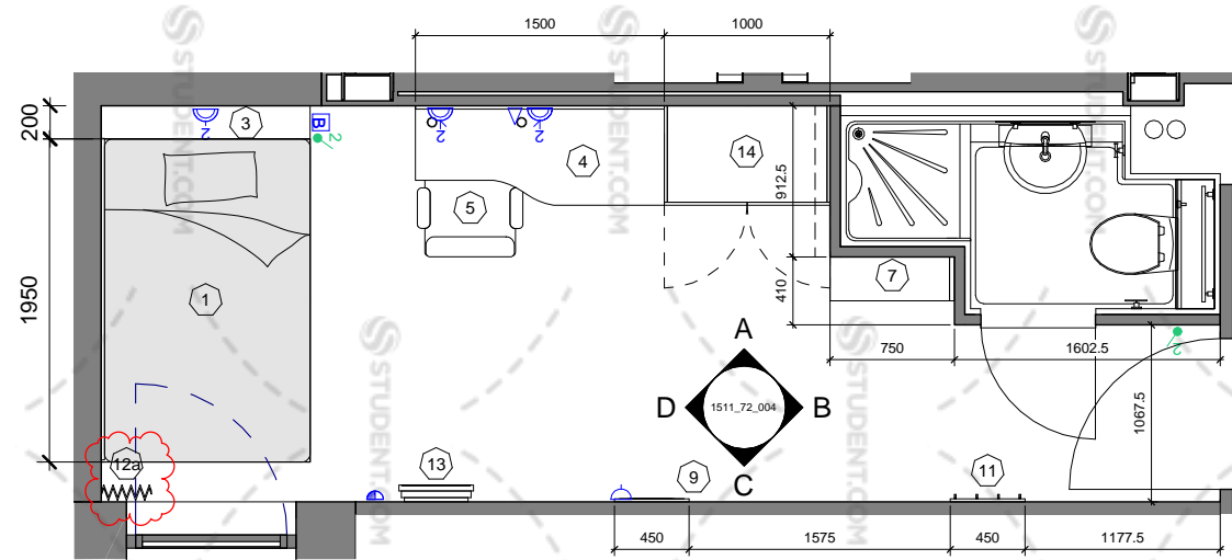
SB_4 - Plan View
