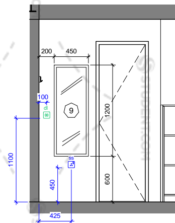
Elevation C
