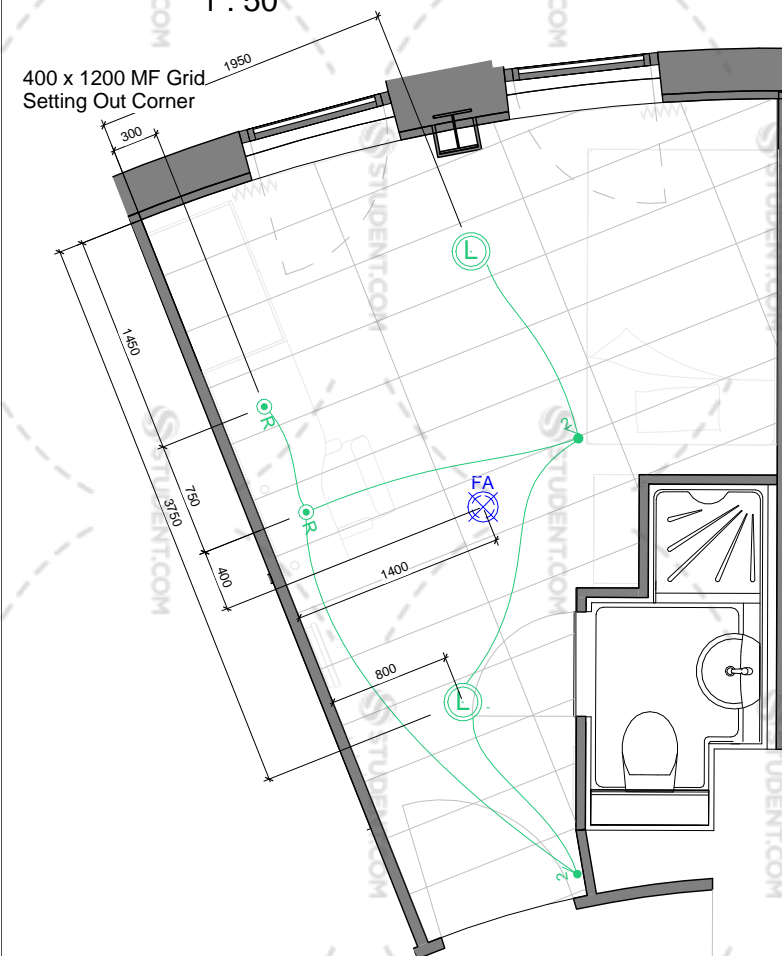
SB_3 - Reflected Ceiling Plan
