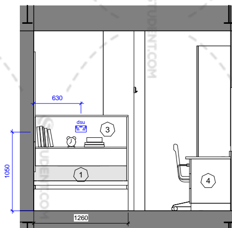
SB_5 - Elevation D
