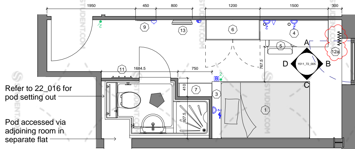
SB_5 - Plan View
