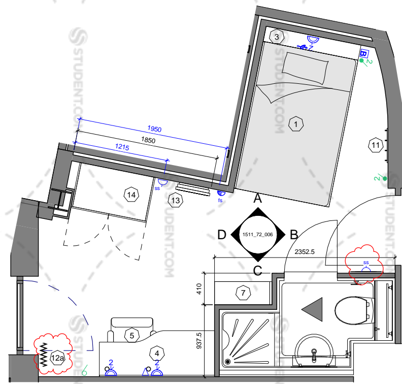
SB_6 - Plan View
