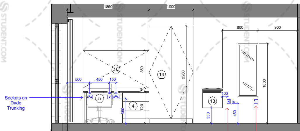
SB_8 - Elevation A
