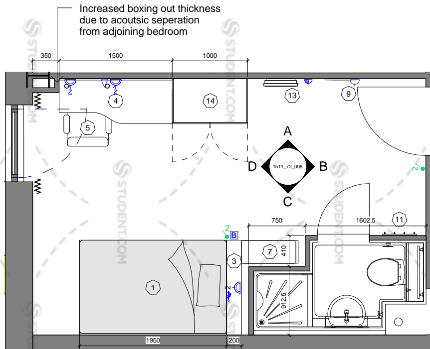
SB_8 - Plan View
