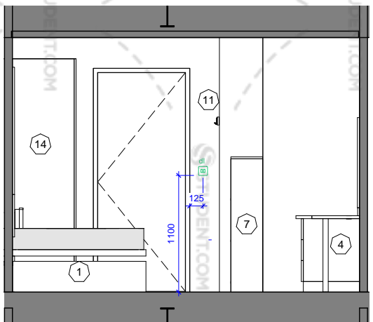
SB_2 - Elevation D 1 : 50
