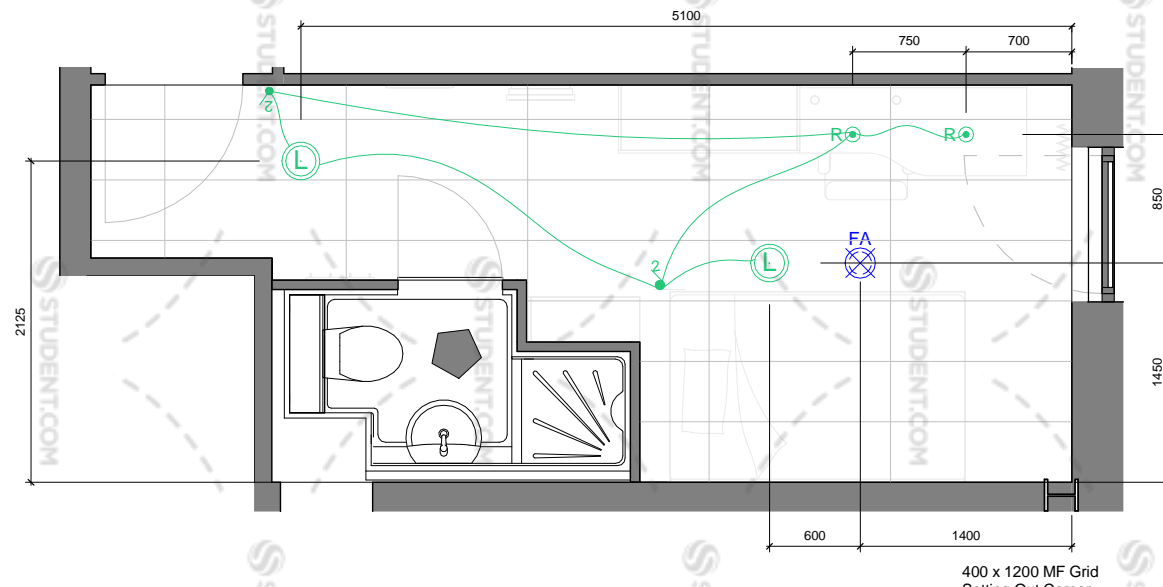
SB_5 - Reflected Ceiling Plan
