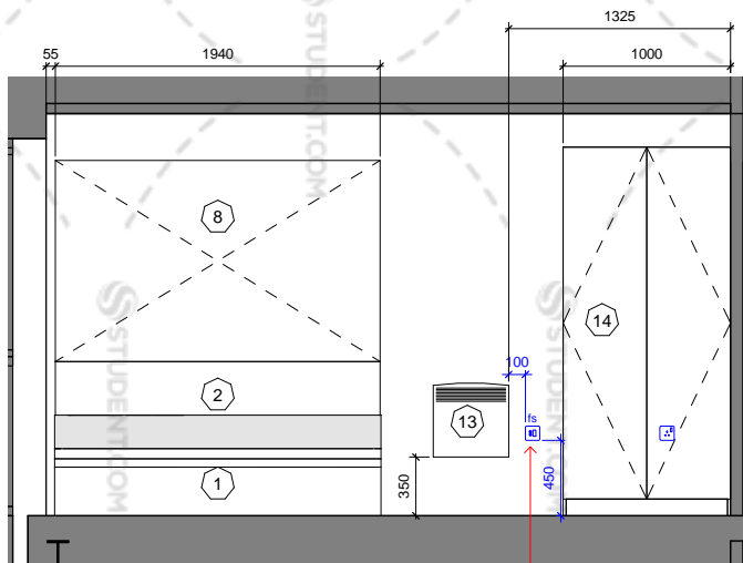
SB_2 - Elevation C 1 : 50
