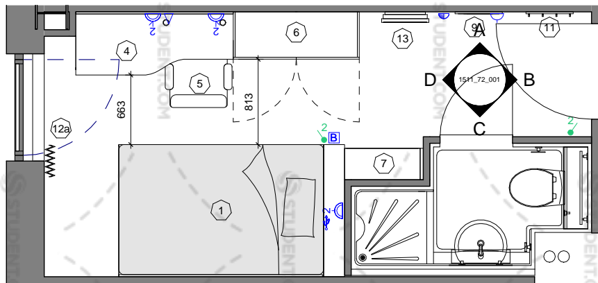
SB_1 - Plan View
