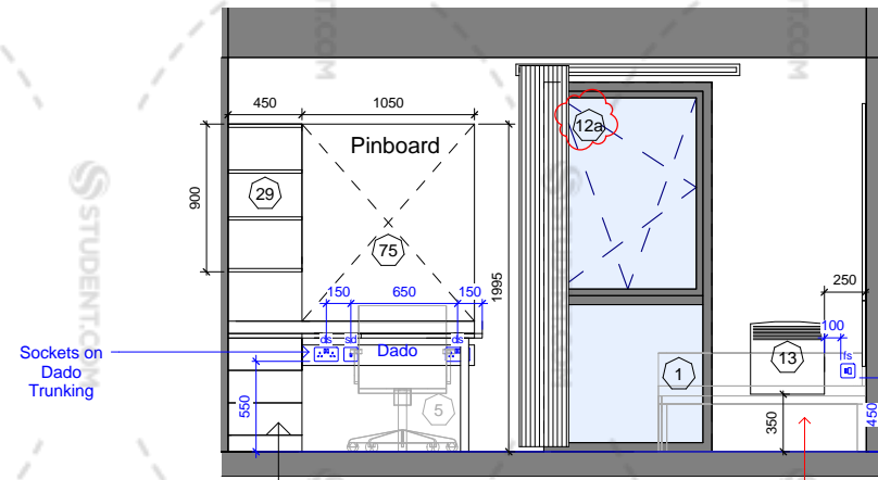
SB_11 - Elevation B
