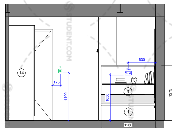
SB_8 - Elevation B
