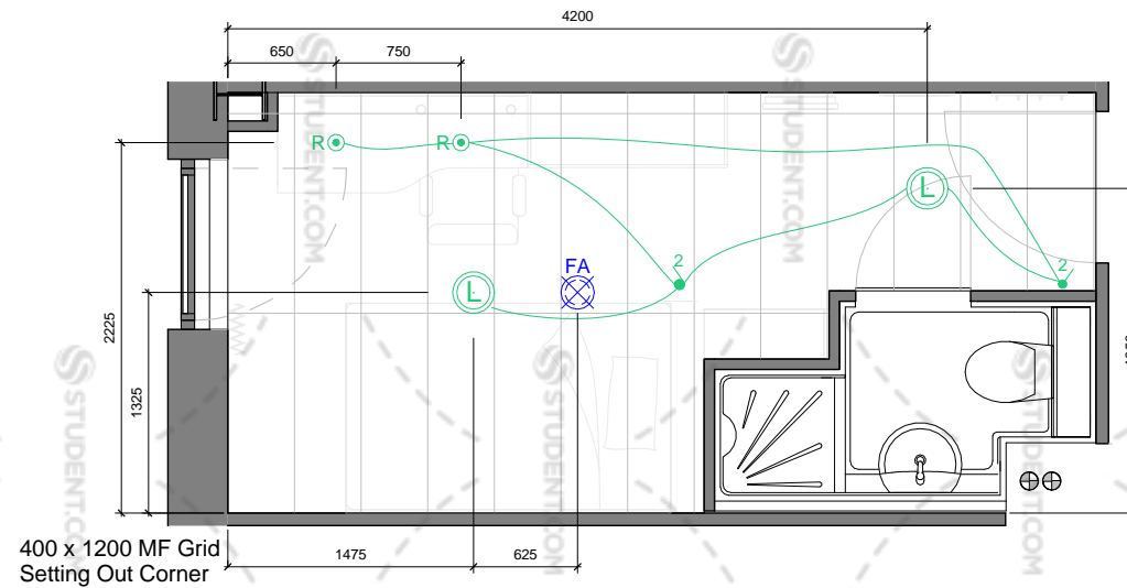
SB_1 - Reflected Ceiling Plan
