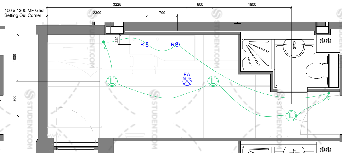
SB_4 - Reflected Ceiling Plan
