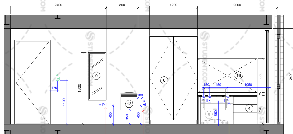
SB_5 - Elevation A
