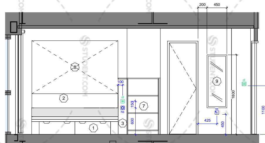
SB_3 - Elevation A
