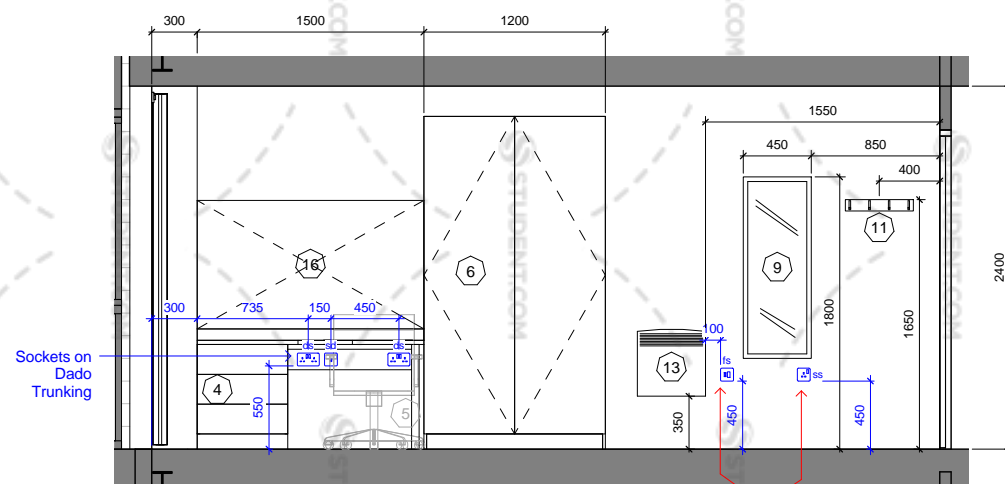
SB_1 - Elevation A
