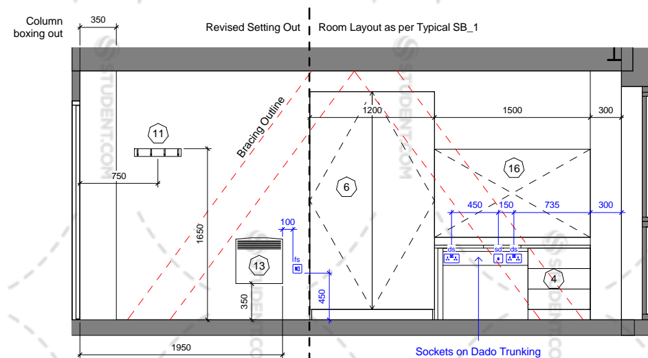
Elevation B - Right Hand Room 1 : 50
