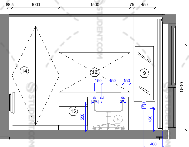
SB_14 - Elevation B 1 : 50
