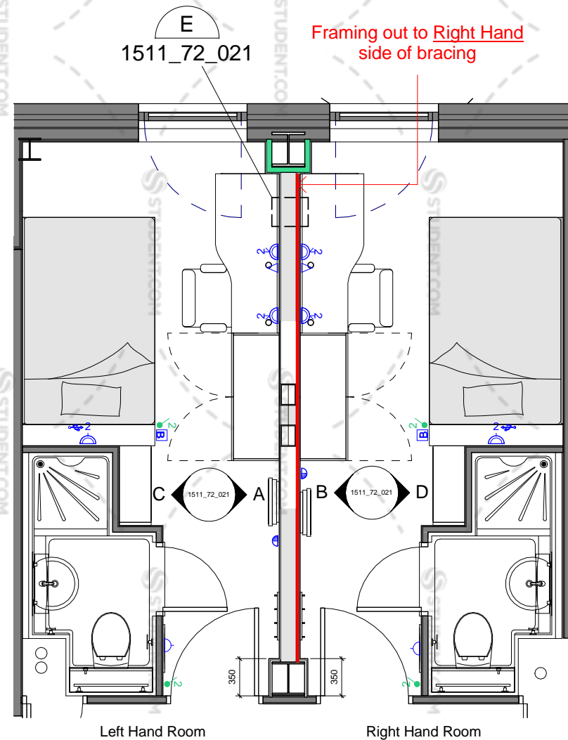
SB_1 - Rooms Next to Bracing 1 : 50
