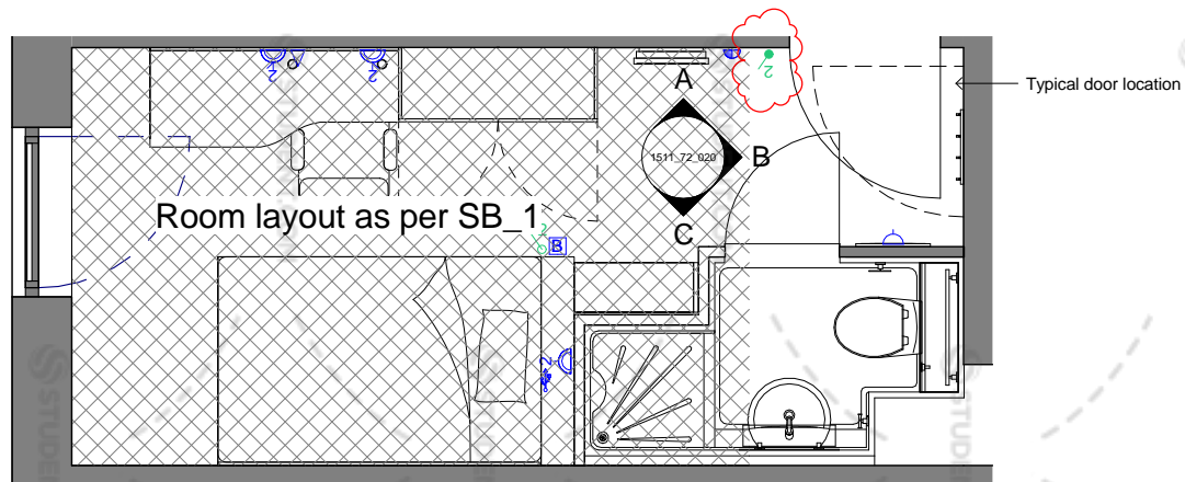
SB_1 - Plan View (Door Variant) 1 : 50
