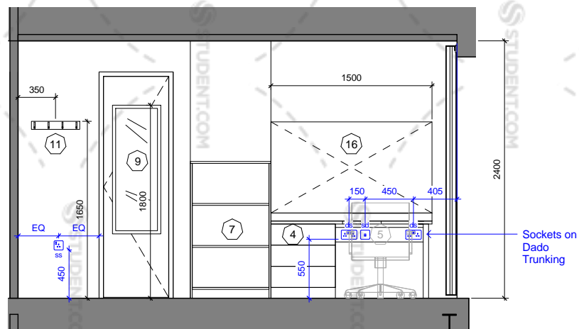
SB_2 - Elevation A 1 : 50
